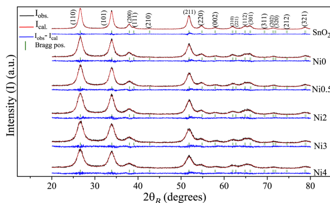
FIG. 1. XRD profiles, along with the Rietveld refinement, of the nanocrystals. The black lines correspond to the observed intensity ( I_{\text{obs}} ), the red lines correspond to the calculated intensity ( I_{\text{cal}} ), horizontal blue lines represent the difference between observed and calculated intensities ( I_{\text{obs}} - I_{\text{cal}} ), and the green vertical ticks correspond to the Bragg positions.
