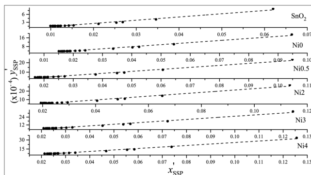
FIG. 2. Size-strain plot for the nanocrystals. The dotted lines represent the linear fits corresponding to the size-strain plots (SSP).
