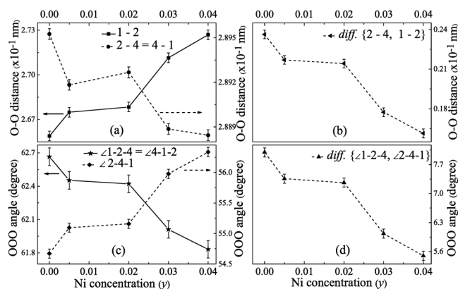
FIG. 17. The variation of various O-O bond parameters with Ni codoping concentration ( y ). The syntax diff {quantity1, quantity2} stands for the difference between quantity1 and quantity2 . The solid and dotted lines are eye guides.
