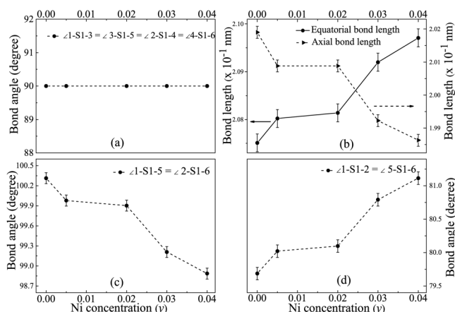
FIG. 16. The variation of various Sn-O bond parameters, in Sn octahedral coordination geometry, with Ni codoping concentration ( y ). The solid and dotted lines are eye guides.
