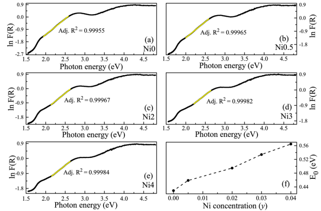
FIG. 10. The plots for Urbach-type absorption [according to Eq. (2) in the nanocrystals] (a)–(e) and variation of the E_0 with Ni concentration ( y ) (f). The solid yellow lines in (a)–(e) represent the corresponding linear fits, whereas the dotted line in (f) is for an eye guide.
