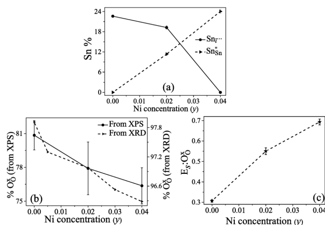
FIG. 14. Variation of % of Sn_i^{''} and Sn_{Sn}^{''} in the total Sn concentration (a), % of lattice oxygen ( O_O^x ) as obtained from O 1s core-level XPS and Rietveld refinement of XRD spectra (b), and the ratio of the concentration of surface state to that of lattice oxygen ( E_s : O_O^x ) (c) with Ni doping concentration. All the solid and dotted lines are eye guides.
