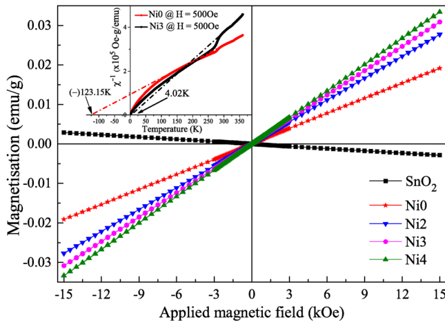
FIG. 13. Room temperature response of the magnetization ( M ) toward the applied magnetic field ( H ) for the nanocrystals. The inset figure shows the temperature dependent magnetization ( M ) curves for the Ni0 and Ni3 nanocrystals. The dashed-dot lines in the inset figure represents the corresponding Curie-Weiss fits.
