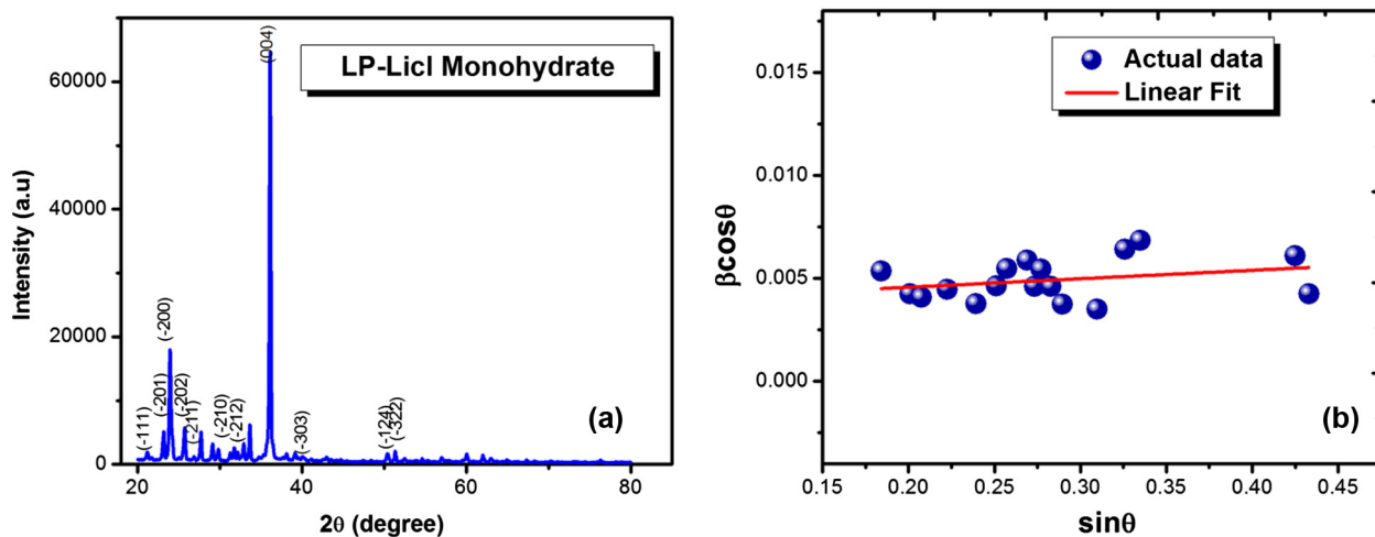
Figure 2 Powder X-ray diffraction pattern along with \beta \cos \theta versus \sin \theta plot.
