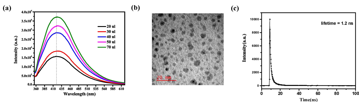
Figure 2. (a) PL spectra of CQD aqueous solution at excitation wavelength of 320 nm (b) TEM image of CQDs (c) PL decay curve of CQDs
