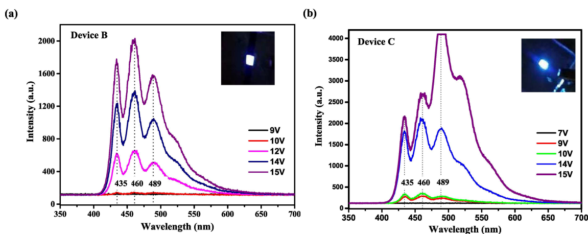
Figure 4. Electroluminescence spectra of OLEDs as function of operating voltage (a) Device B: ITO/PEDOT:PSS/PFO/LiF/Al (b) Device C: ITO/PEDOT:PSS/PFO/CQD/LiF/Al (inset shows brightness of OLED at 15 V)
