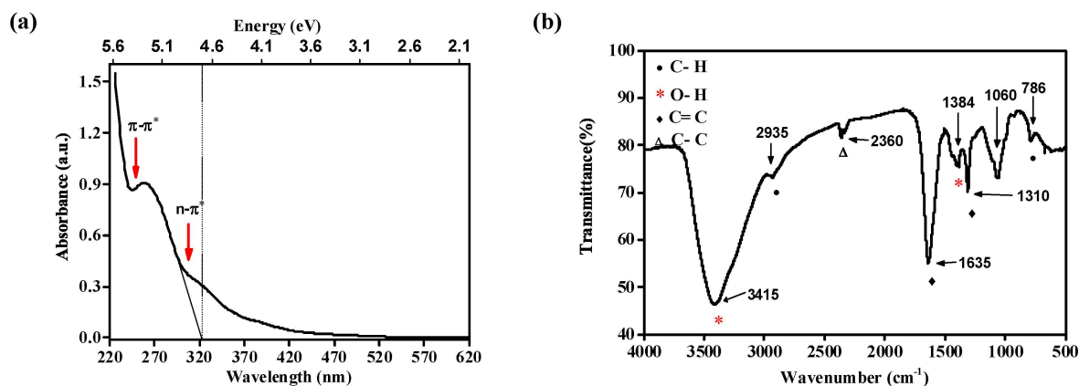
Figure 1. (a) UV-Vis absorption spectra of CQD in aqueous solution and (b) FT-IR spectrum of CQDs, showing characteristic
