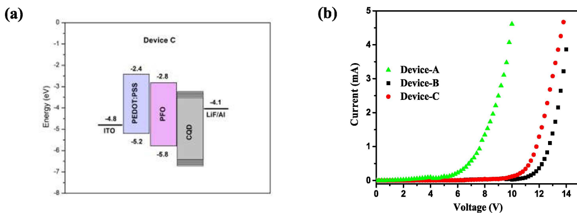
Figure 3. (a) Schematic diagram of energy level alignment of OLEDs (b) Current Voltage Characteristics of OLEDs (Device-A - ITO/PEDOT:PSS/CQD/LiF/Al; Device-B - ITO/PEDOT:PSS/PFO/LiF/Al and Device-C - ITO/PEDOT:PSS/PFO/CQD/LiF/Al)
