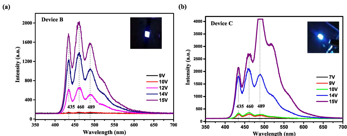
Figure 5. Electroluminescence spectra of OLEDs as function of operating voltage (a) Device B: ITO/PEDOT:PSS/PFO/LiF/Al (b) Device C: ITO/PEDOT:PSS/PFO/CQD/LiF/Al (inset shows brightness of OLED at 15 V)
