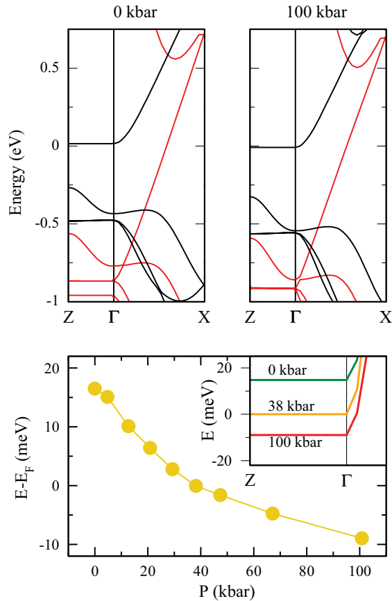
FIG. 10. (Color online) Upper panels: energy bands of LaCoPO at ambient P and at 100 kbar ( E_F = 0 ). The black (red) color refers to majority (minority) spin bands. Lower panel: difference between the energy at \Gamma and the Fermi energy E_F for the band crossing the Fermi energy. Inset: energy band dispersion for selected P values.
