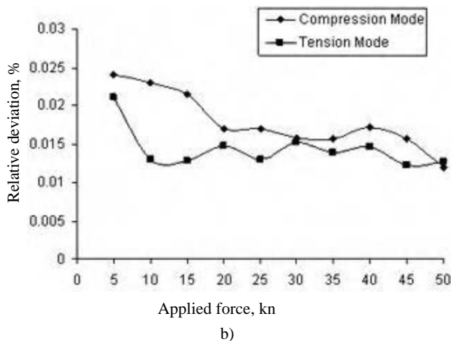
Fig. 5 — Uncertainty of measurement: a) 20 kN FT; and b) 50 kN FT
