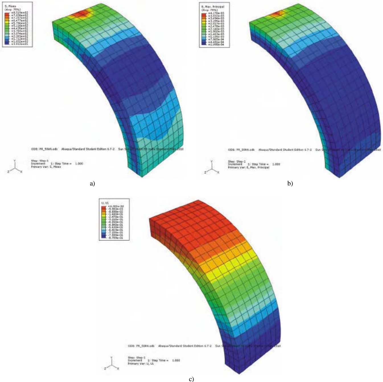
Fig. 2 — Finite element analysis of ring shaped FT under axial applied in tension mode for: a) Stress distribution; b) Strain distribution; and c) Axial deflection
