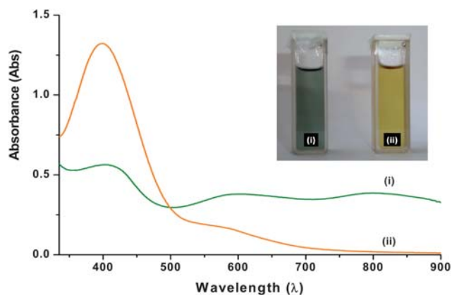
Fig. 3 UV-Visible spectra of CSA doped PANI in (i) formic acid (FA) (ii) ethylene glycol (EG); inset shows visual observation of PANI colloidal suspension in (i) FA (ii) EG.
