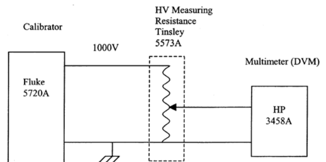
Fig. 2— Schematic diagram for calibration of HV measuring resistance
