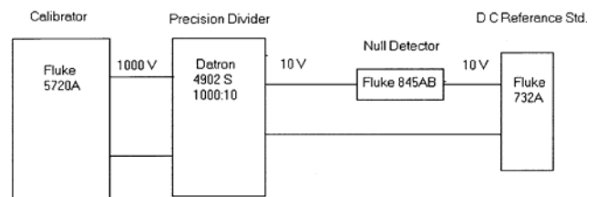
Fig. 1— Schematic diagram for calibration of calibrator
