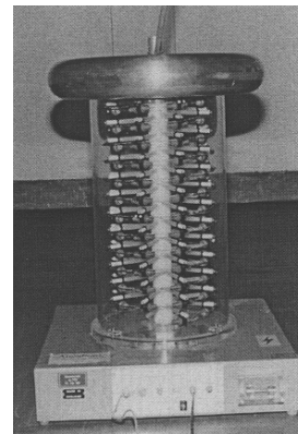
Fig. 5—High Voltage Standard Resistive Divider
