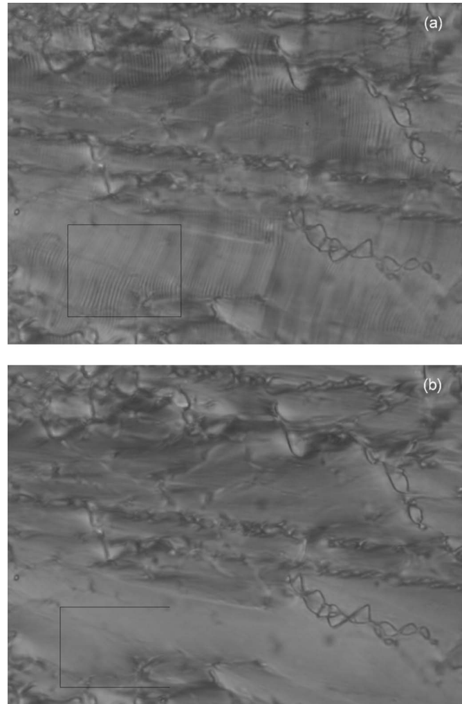
FIG. 3. Optical micrograph of ELC sample cells of 20\ \mu\text{m} thickness at different temperatures of (a) 27^\circ\text{C} and (b) 29^\circ\text{C} . Dechiralization lines are visible at 27^\circ\text{C} (square marked) showing that the phase is Sm-C* but after T_c no lines are seen at 29^\circ\text{C} suggesting that change from Sm-C* to Sm-A phase has taken place.
