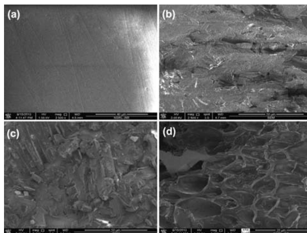
Fig. 5 — SEM images of (a) pure acrylic resin and its composites containing (b) 1 wt%, (c) 10 wt % and (d) 30 wt % of AC
